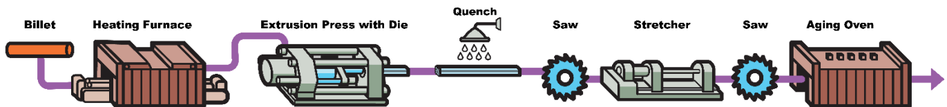
Figure 1. Extrusion manufacturing process schematic
